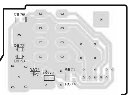
OPERATION (3) P.C.B. (Side B)
